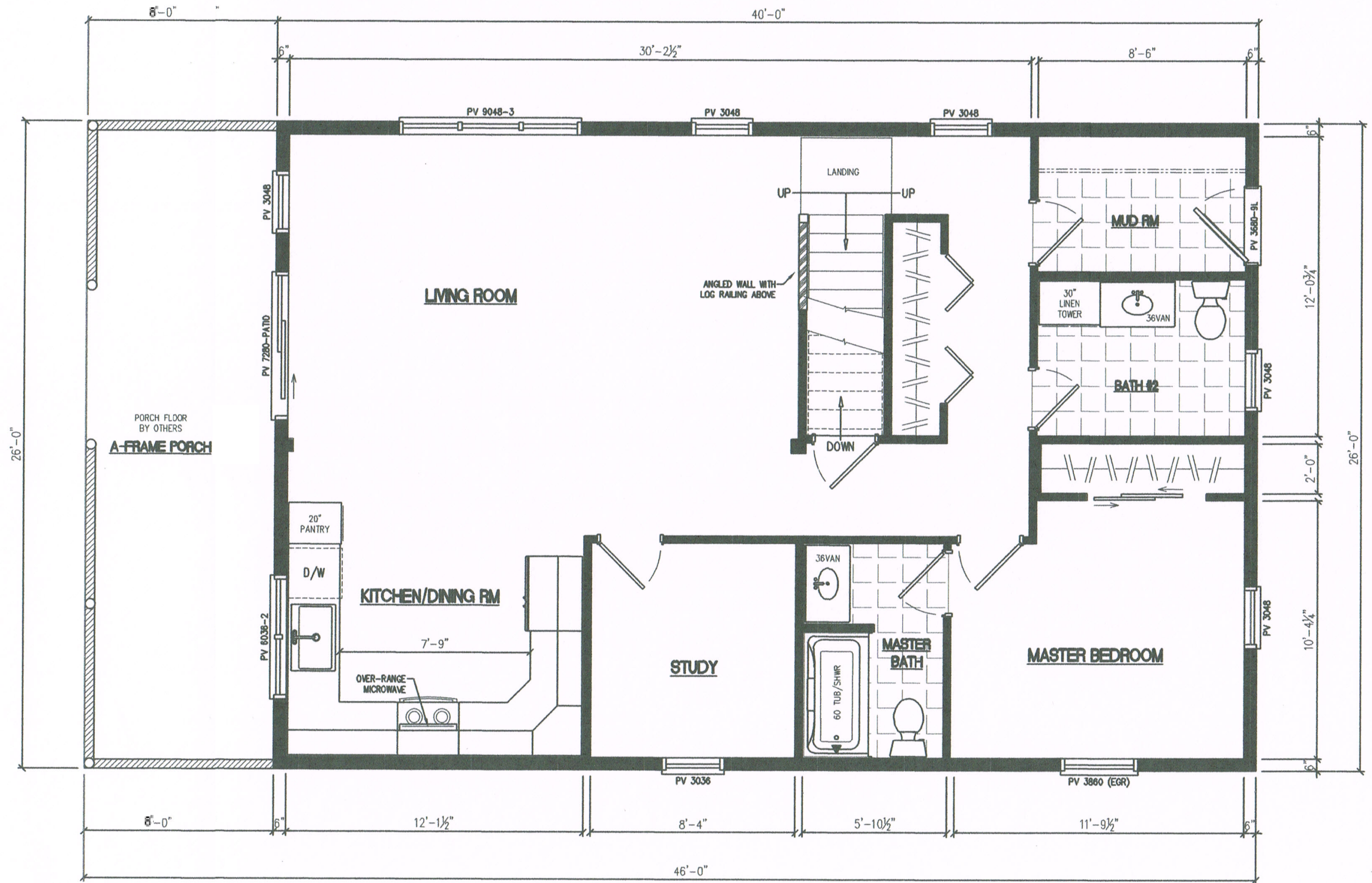
Avon Alternate Plans 1/4" = 1' 0"
