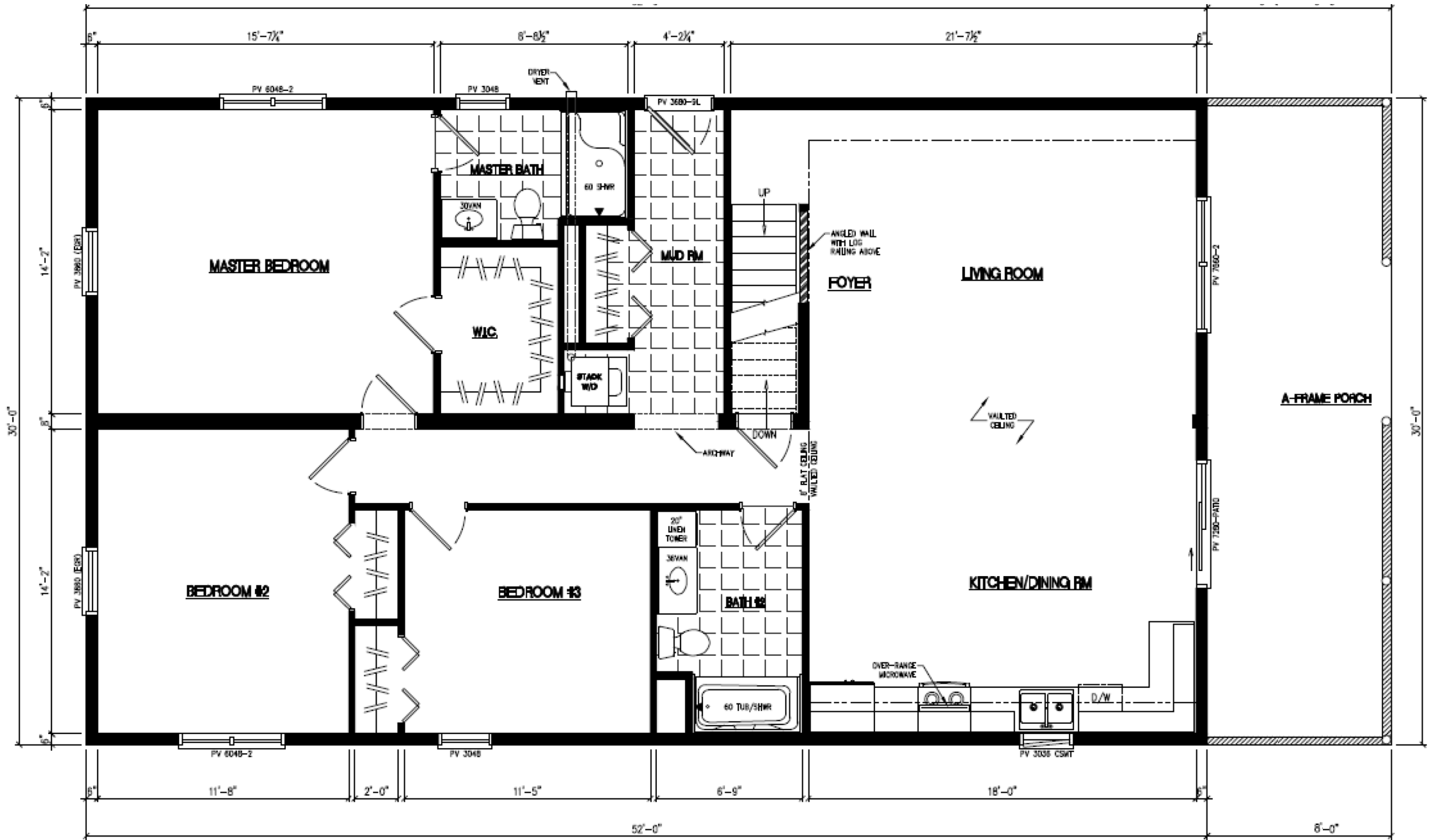
Tarn Plans 1st Floor 1/4" = 1' 0"
