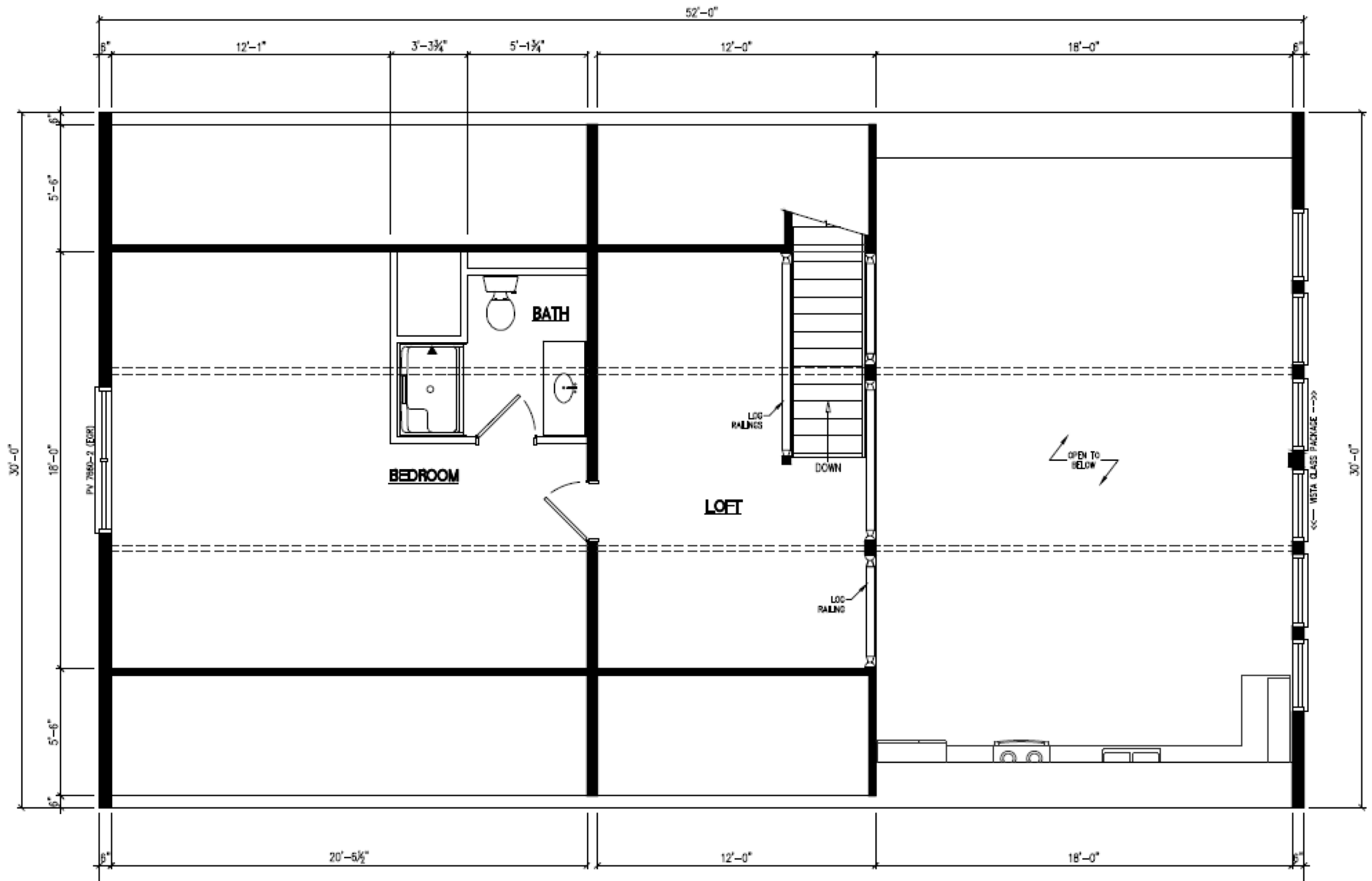
Tarn Plans 2nd Floor 1/4" = 1'0"
