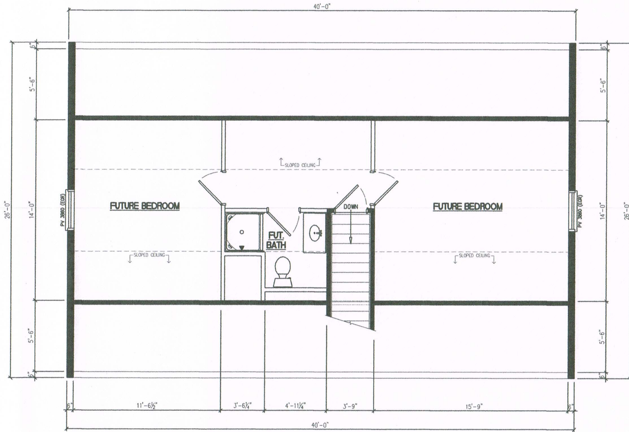
The Avon 2ND Floor 1/4" = 1' 0"
