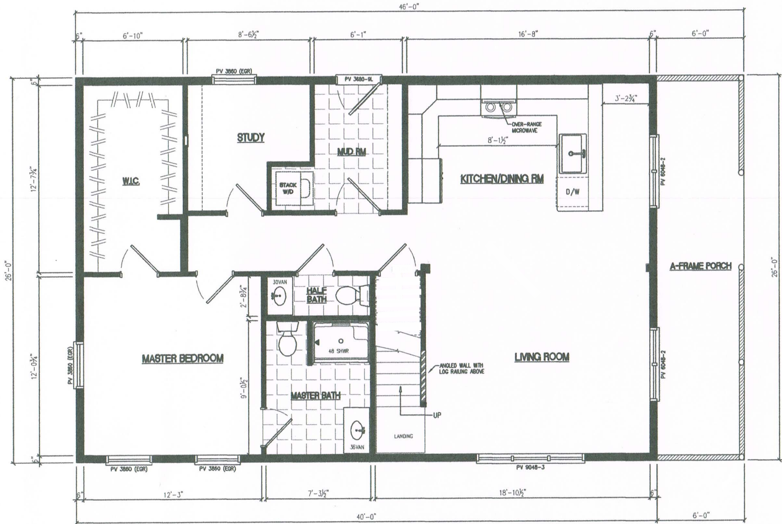
The Avon 1ST Floor 1/4" = 1' 0"
